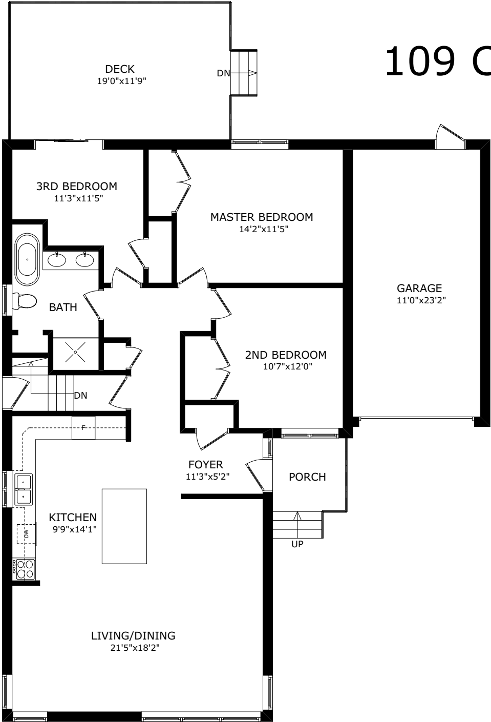
MAIN FLOOR
